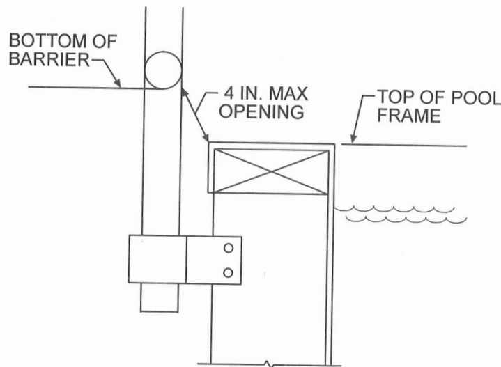
Figure AG105.2(1) OPENING LIMITATIONS
